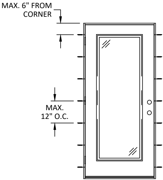
ANCHOR LAYOUT
