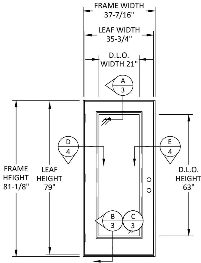
TYPICAL ELEVATION
