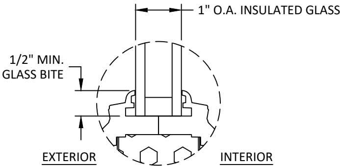
GLAZING DETAIL
